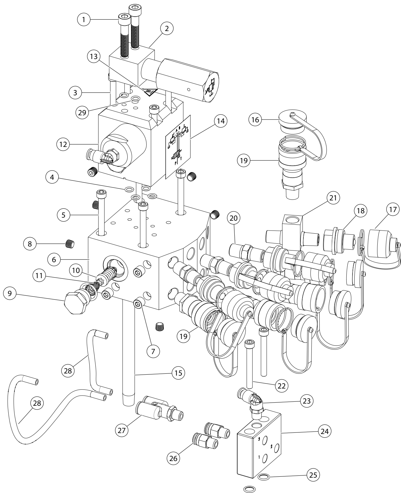
Control Valve & Manifold FMP & FMPR
