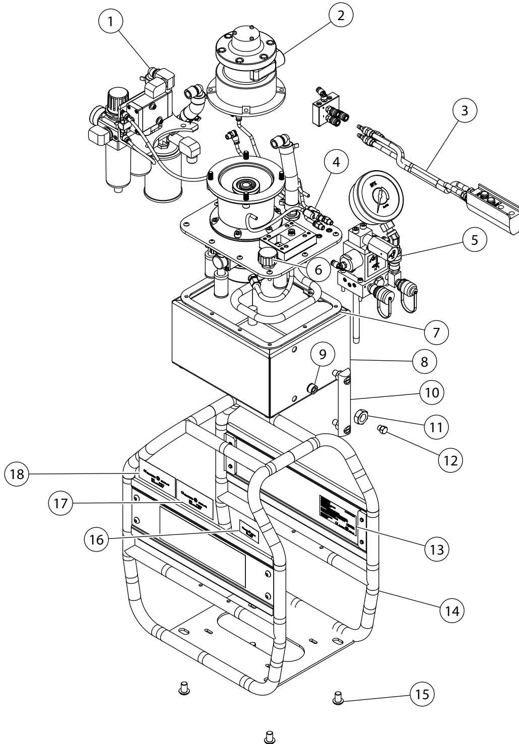
Air Hydraulic Pump PA60APF5FPR
