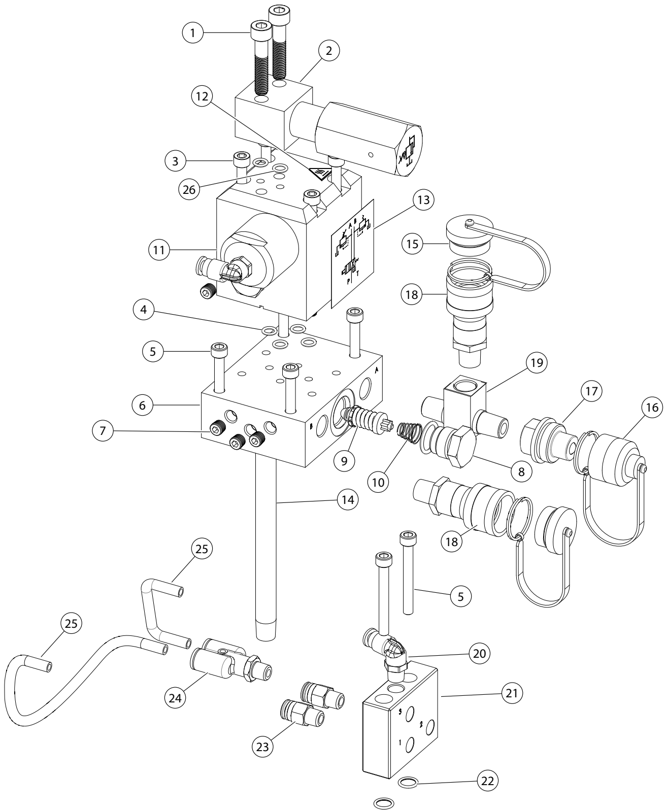
Control Valve & Manifold FP & FPR
