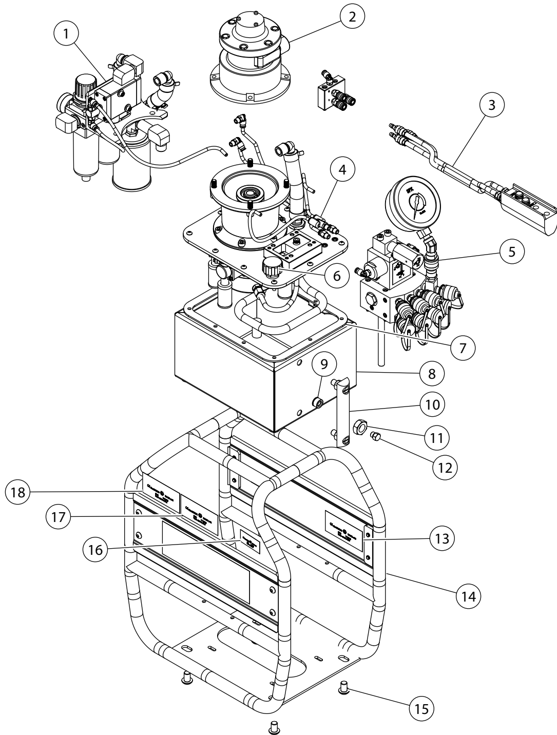
Air Hydraulic Pump PA60APF5FMPR
