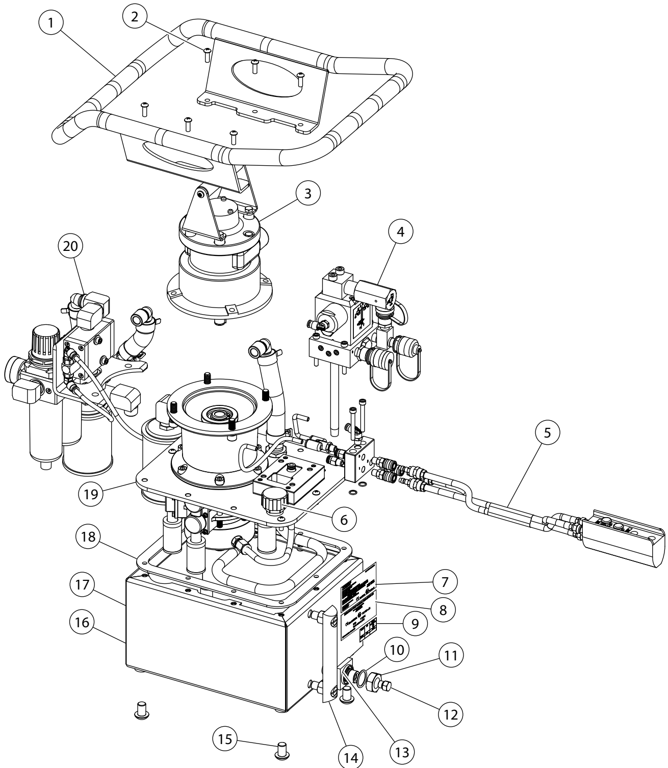
Air Hydraulic Pump PA60APF5FP
