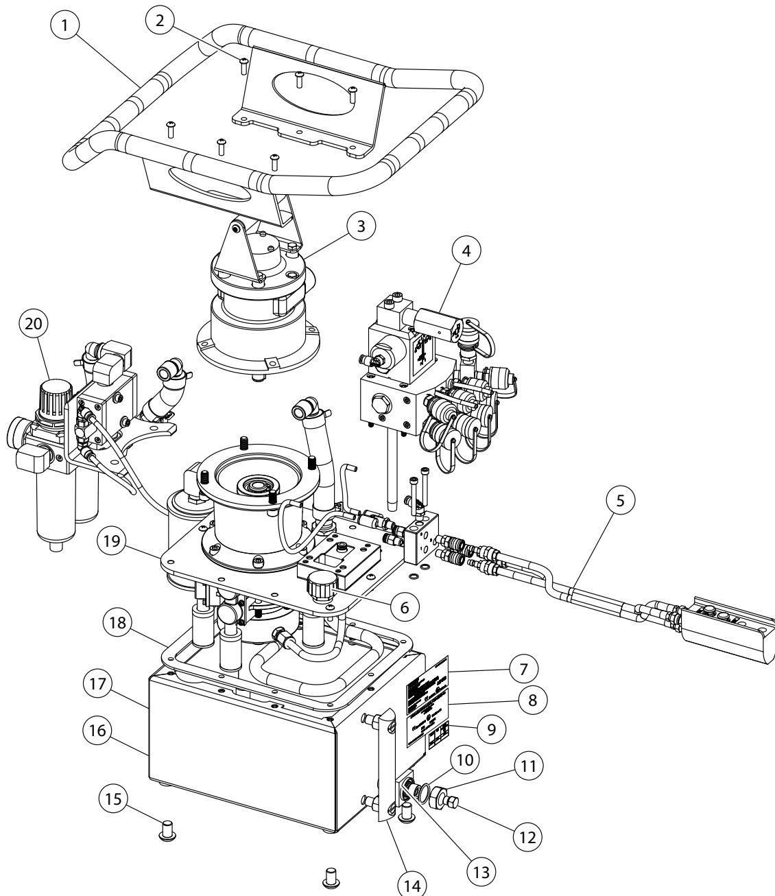
Air Hydraulic Pump PA60APF5FMP
