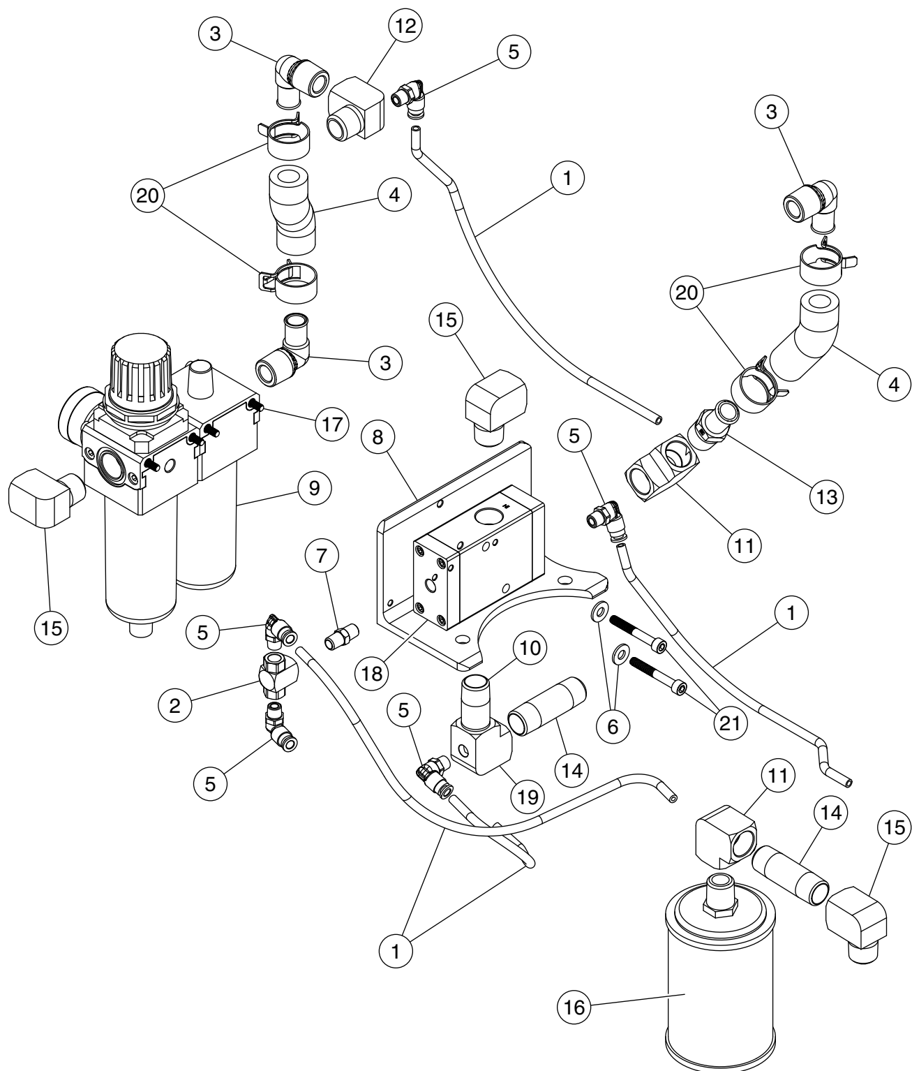
Filter-Regulator-Lubricator & Muffler
