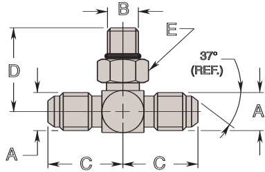
Male Branch Tee 37° Flared Tube to O.R.B.
